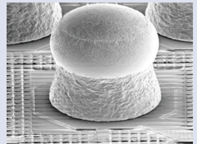
Thick negative tone resist stripping on Cu pillar with SnAg
