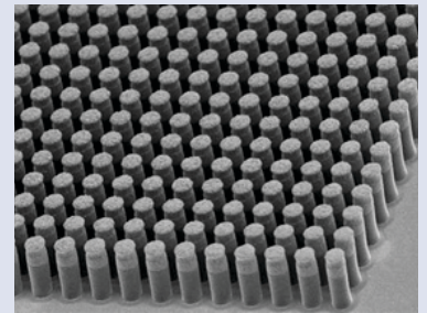
Thick negative tone resist stripping on 70µm copper pillars
