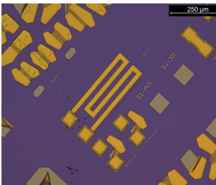
Stripper 2 (70°C, 50 min) Partial removal
