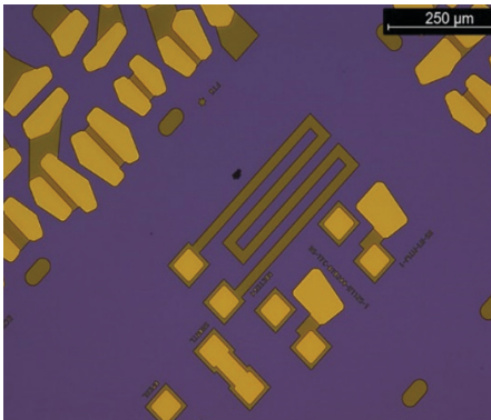
Prior to application of strippers
