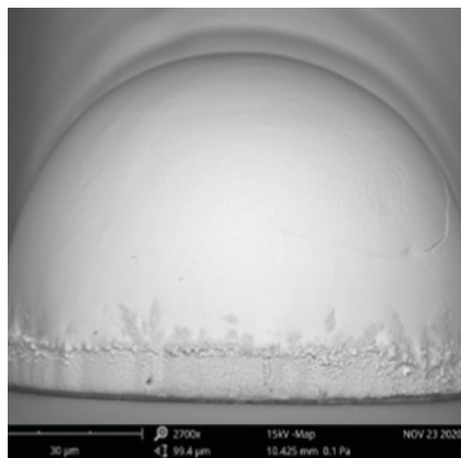
A clearly defined and uniform reflow shown using Elevate ® Tin 5011
