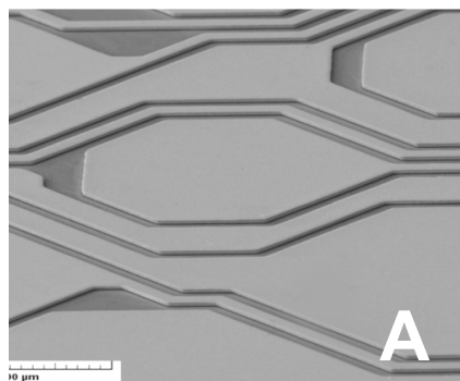
Image 1 shows a typical deposit from a standard sulfite gold bath. Image 2 shows the smooth deposit of Elevate Gold 7990 NBV HT. Image 3 shows Elevate Gold 7990 NBV HT bright deposit appearance.
