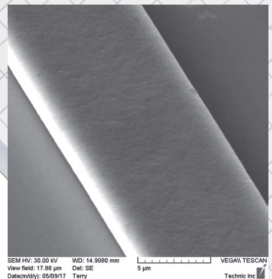
10 micron line with 2 microns of Elevate® Ni 5950 Ra of 7 nm
